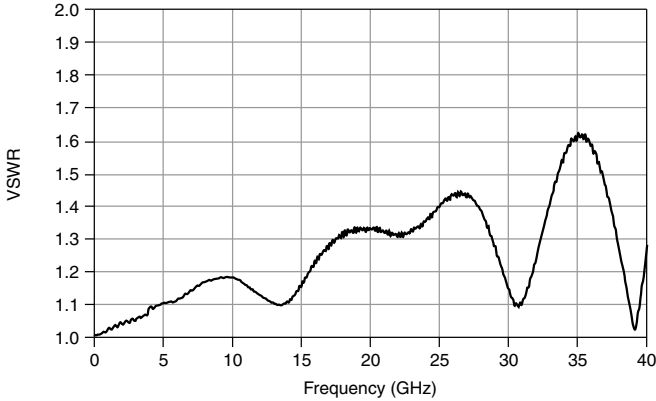
Figure 3. Typical VSWR
