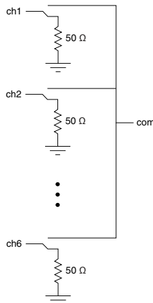
Figure 4. NI 2797 Power-On State
