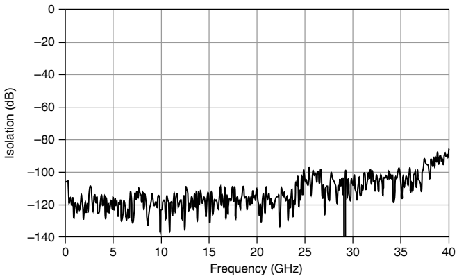
Figure 2. Typical Isolation
